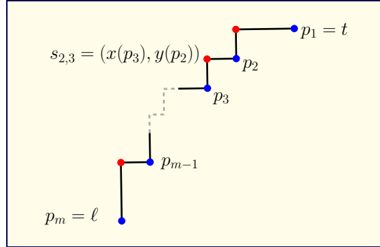
Figure 4.4: Construction of the chain C_{t\ell} from a given convex point set (blue color).
