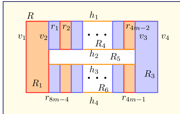
Figure 6.6: Structure of a variable gadget.
