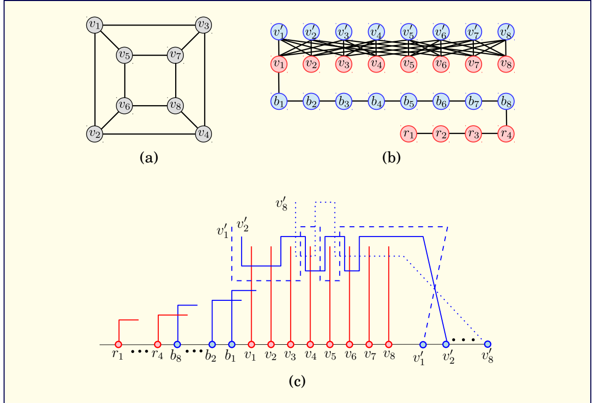
Figure 8.4: (a) A graph G . (b) Construction of H from G with k = 4 . For the clarity of the figure we omit the edges between each pair of vertices v'_i and v'_j , for i \neq j . (c) Intersection model of H .
