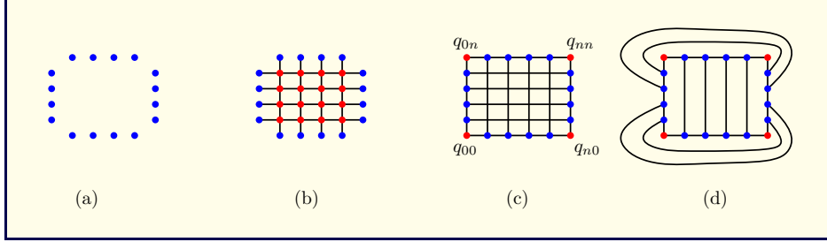
Figure 4.1: Blue circles represent the points in P , and red circles represent Steiner points. (a) The point set P , (b) construction of a plane Manhattan network for the point set P , (c) a planar Manhattan network G^* of P , and (d) a planar embedding of G^* where the curved edges have weight/length n .
