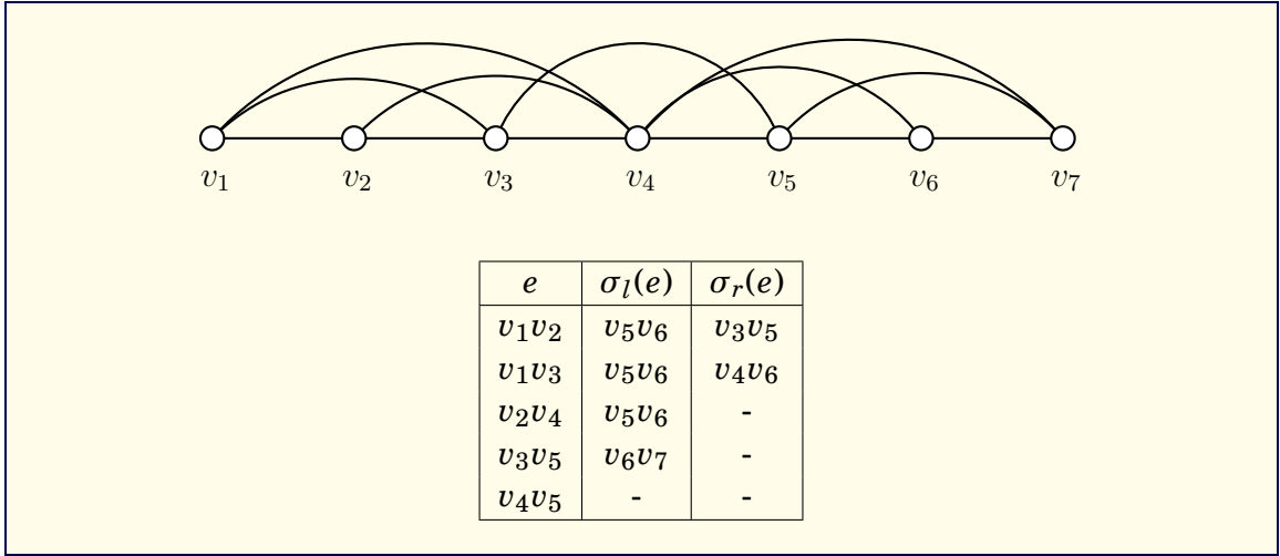
Figure 7.2: Example of an proper interval graph shown with vertices arranged according to the proper vertex ordering v_1, v_2, \dots, v_7 . The table shows some edges and their left and right successors. Where a particular successor does not exist for an edge, the corresponding entry is marked as “-”.
